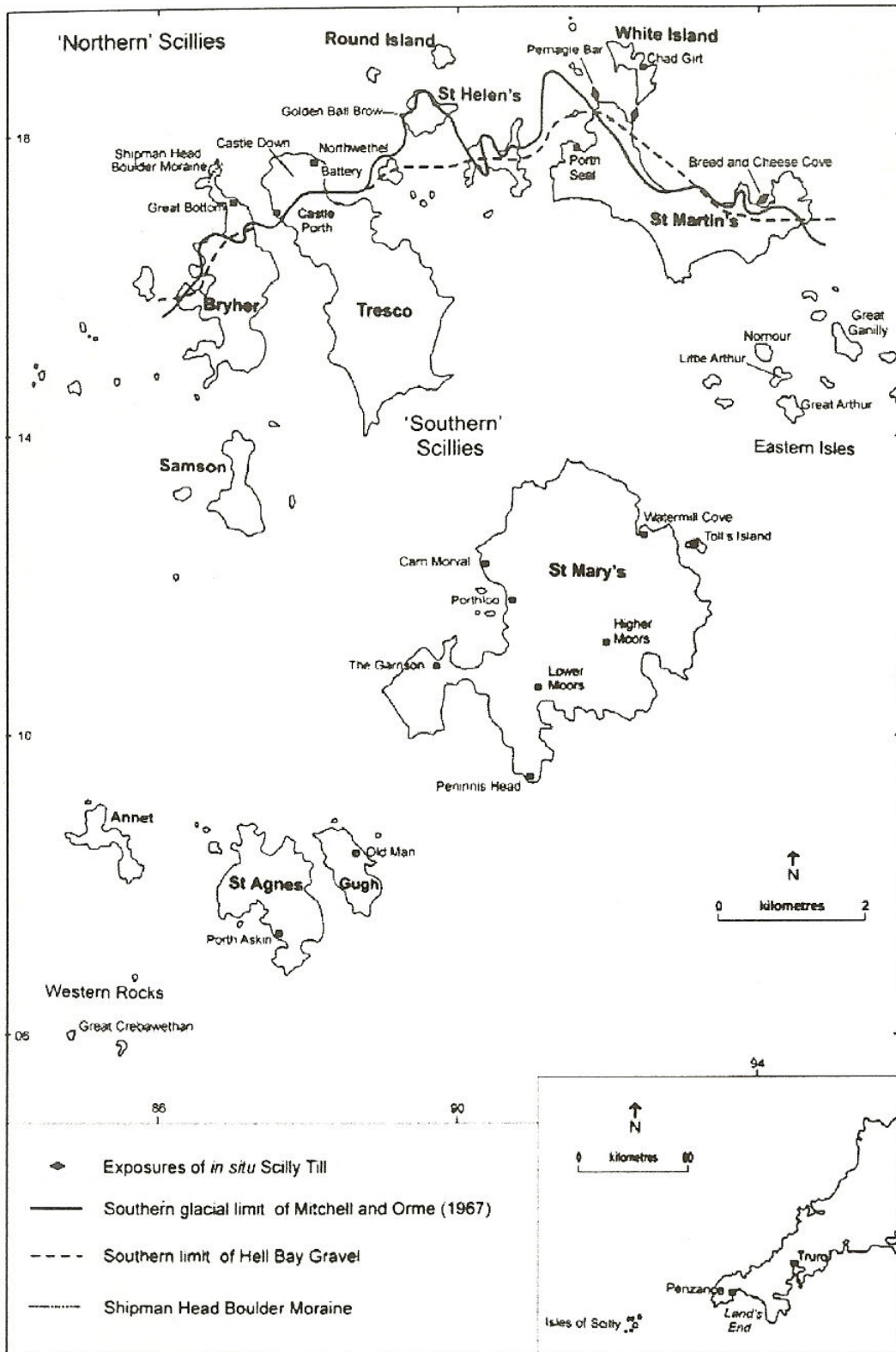
Figure 1: The Isles of Scilly: map showing location of sites mentioned in the text, and ice limits and moraine positions.
